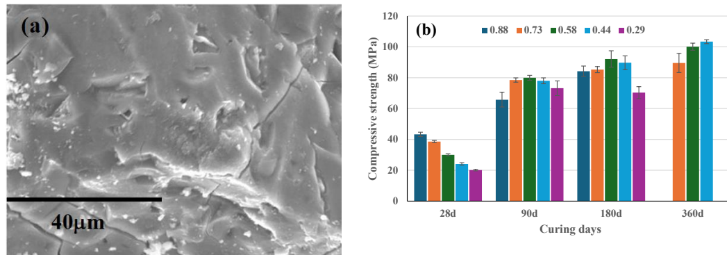
Figure 1. (a) SEM micrograph of 0.44 paste after 360 days; (b) Compressive strength development of alkali-activated mortars based on VCAS with different \text{SiO}_2/\text{Na}_2\text{O} molar ratios (from 0.88 to 0.29).
