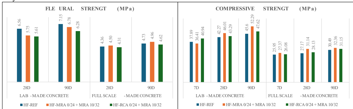
Figure 1. Flexural strength (Left) and Compressive strength (Right) of Lab-made and Full scale-made recycled concrete
