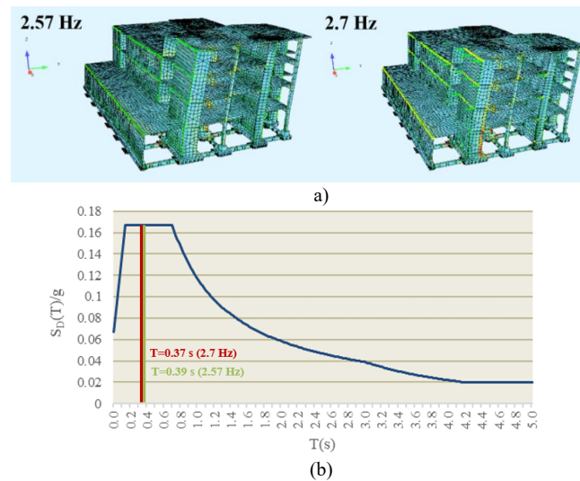
Figure 1. Comparison of the main vibration modes applying various edge stiffnesses. a) Graphical representation of the main vibration modes of the structure for different stiffnesses. b) Response spectrum with the associated periods for different structure stiffnesses
