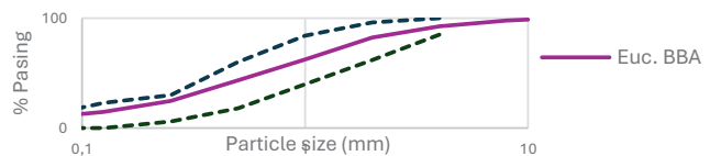
Figure 1: Particle size distribution
